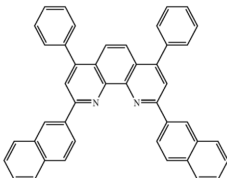
NBphen
