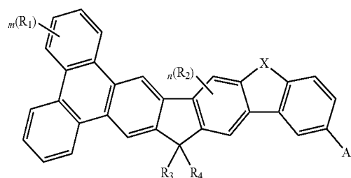
formula(III)
