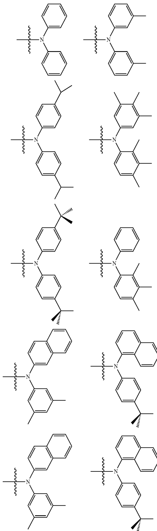
formula(I)
